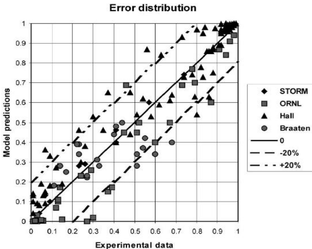
Figure 2.28 - Error distribution of Biasi's model predictions (Biasi et al. , 2001)
