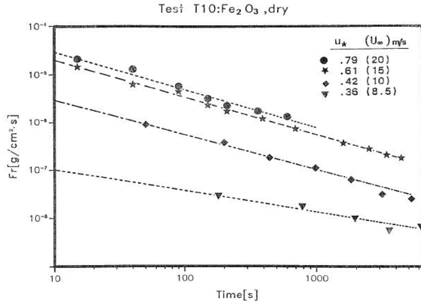
Figure 2.30 - Resuspension flux vs. time of Fromentin's model (Fromentin, 1989)
