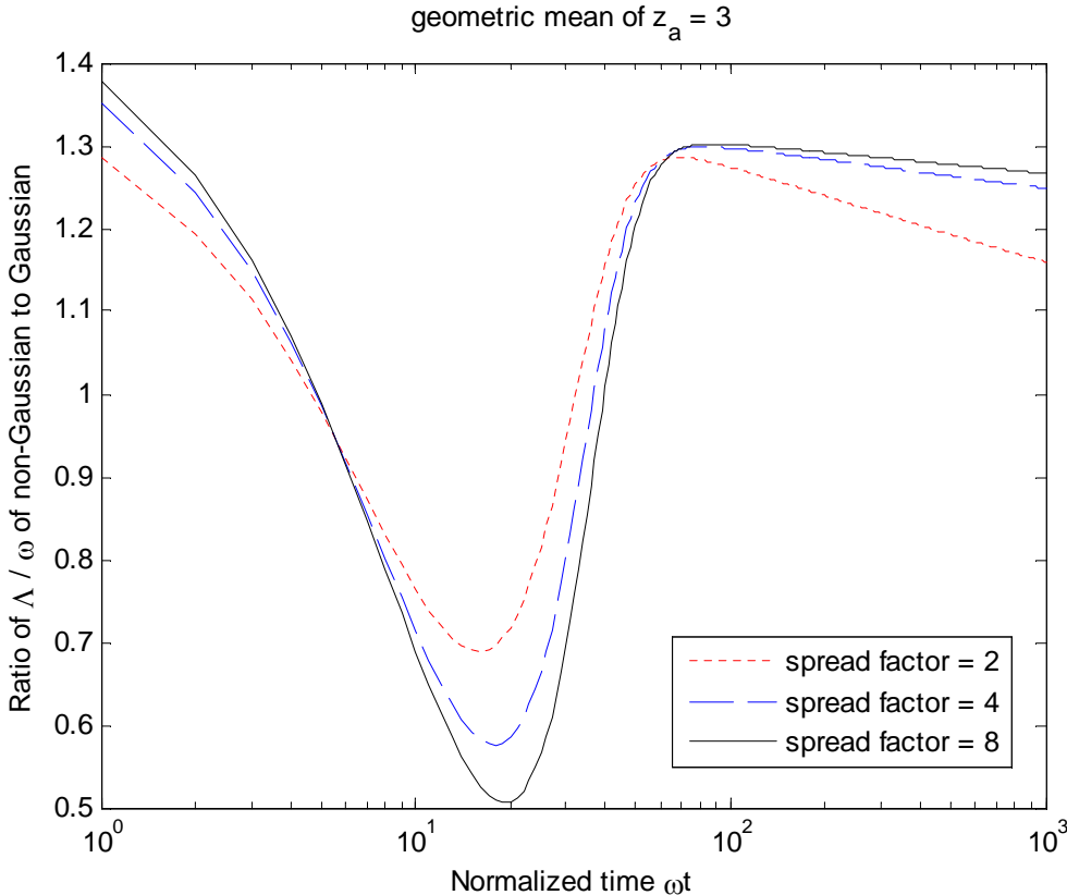
Figure 4.23 - Ratio of normalized resuspension rate of non-Gaussian to Gaussian vs. \omega t ( z_a = 3 )
