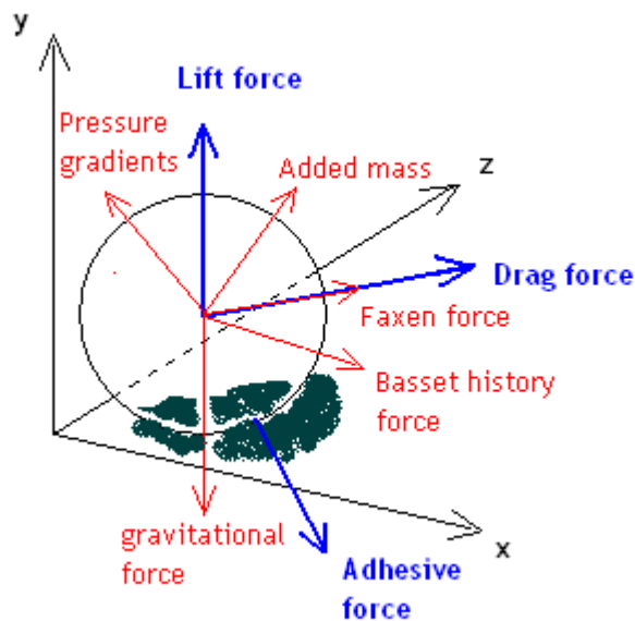
Figure 2.1 - Forces on particle
