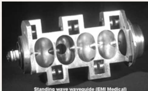
Standing wave waveguide (EMI Medical)
