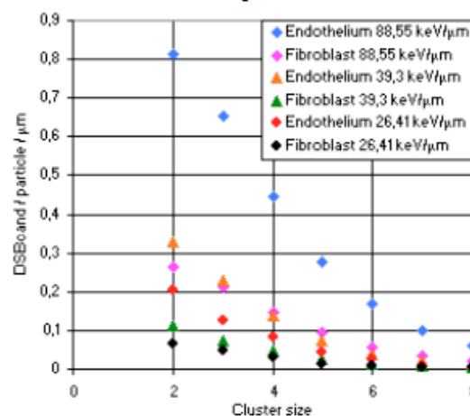
Figure 3. Complexity of DNA clustered damages induced by alphas for three different LET.
